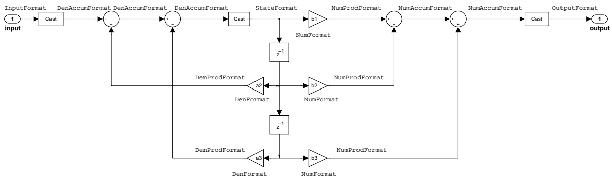
Figure 7-1: df2 IIR Filter Structure Including The Formatting Objects, With Arithmetic Property Value fixed
