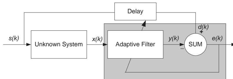
Figure 4-4: Determining an Inverse Response to an Unknown System
